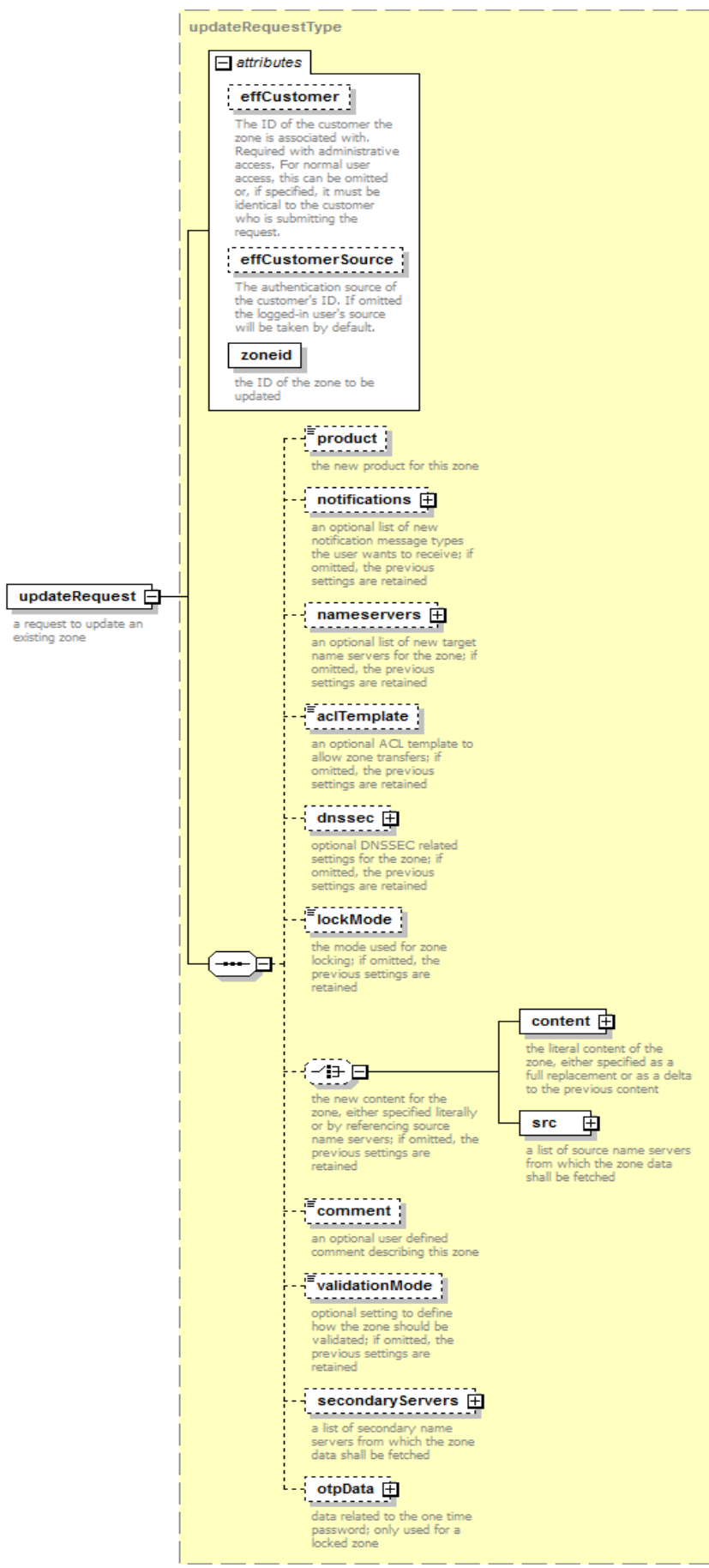
Figure 2: updateRequest schema
